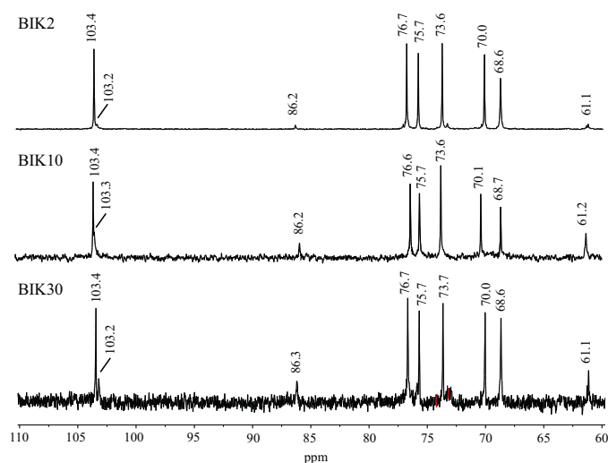
Fig. 2. ^{13}\text{C} NMR spectra of (1 → 6)-β-D-glucans from B. inquinans (Fries).
